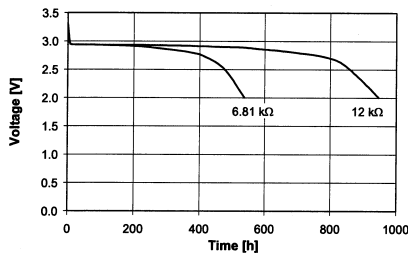
Discharge performance at 23°C
