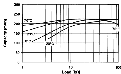
Cell capacity at various loads
