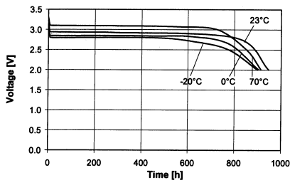
Temperature performance Load 12kΩ
