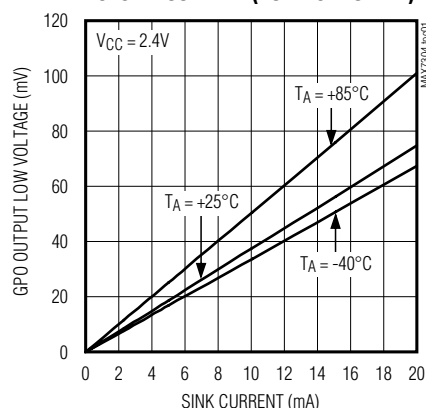
GPO OUTPUT LOW VOLTAGE vs. SINK CURRENT (PORT15–PORT12)
