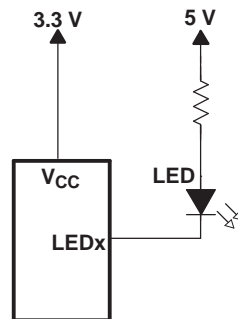
Figure 25. Device Supplied by a Lower Voltage
