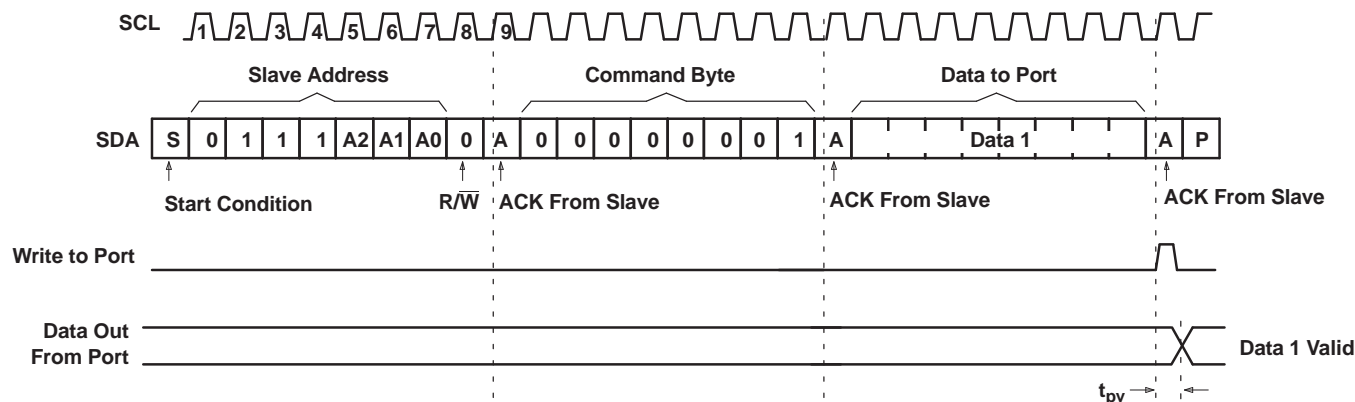
Figure 19. Write to Output Port Register
