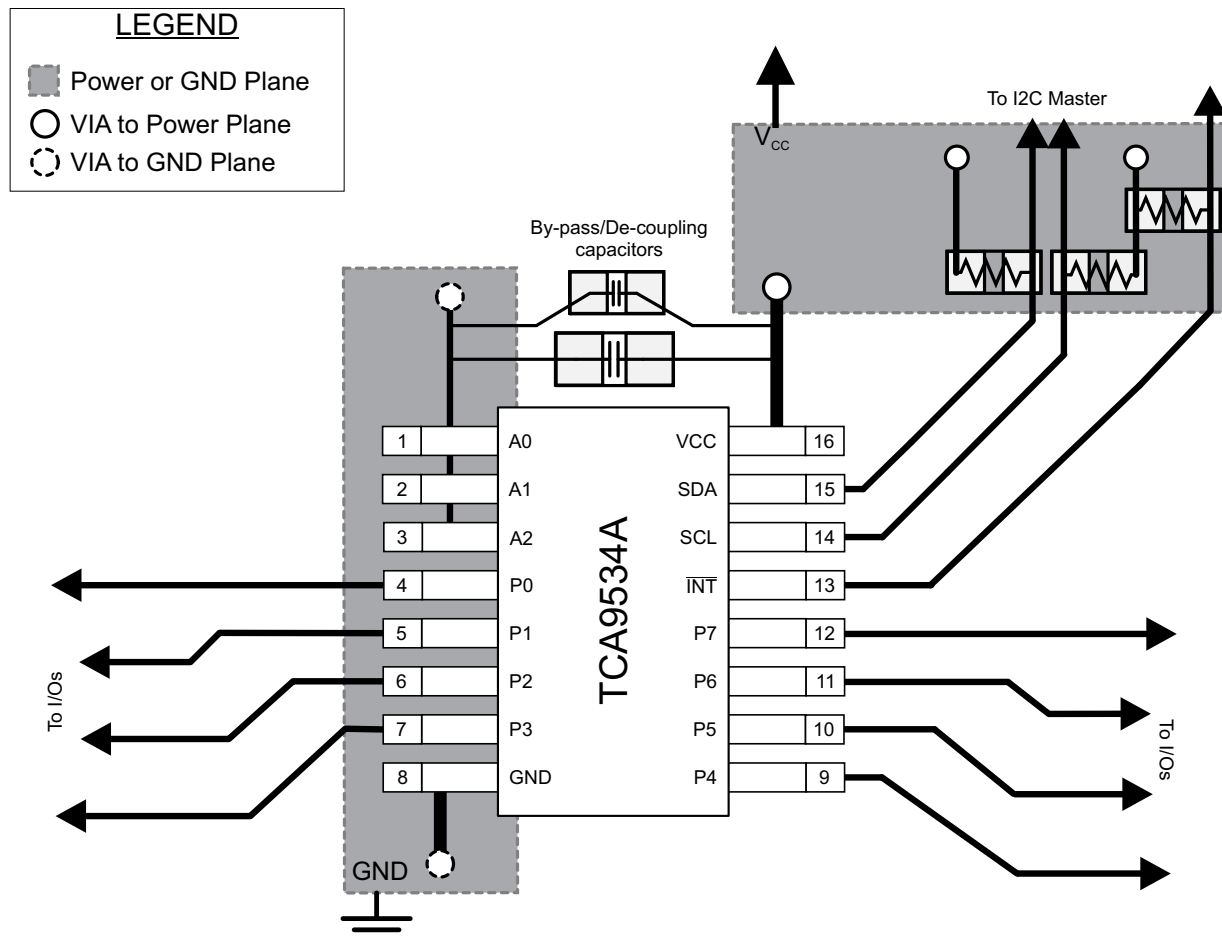
Figure 31. TCA9534A Layout
