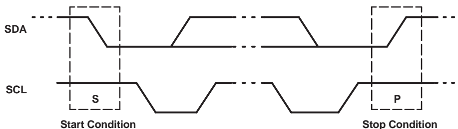
Figure 14. Definition of Start and Stop Conditions
