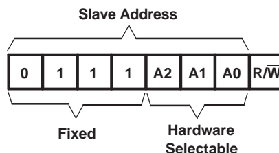
Figure 17. TCA9534A Address
