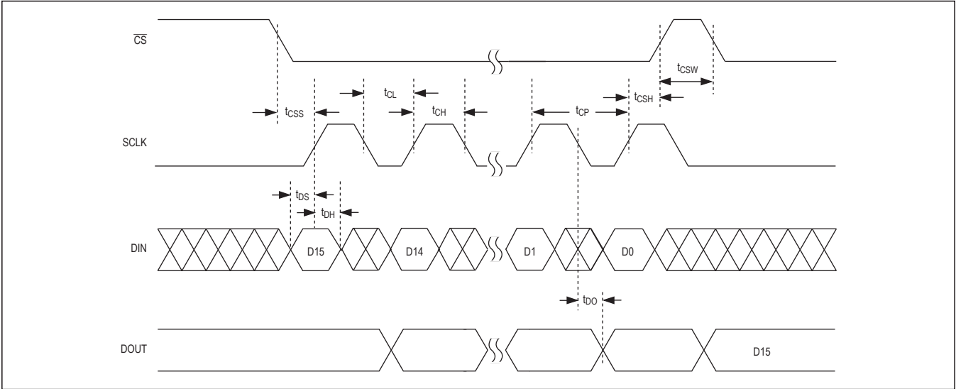
Figure 4. Timing Diagram
